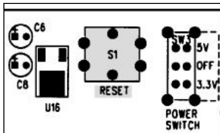
Figure 5: Reset Pushbutton
