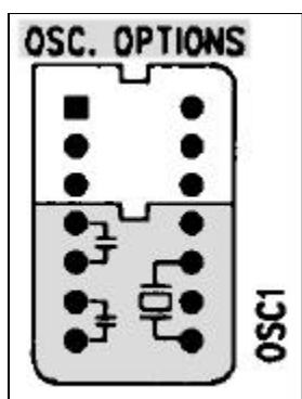
Figure 11: Half-Size Oscillator
