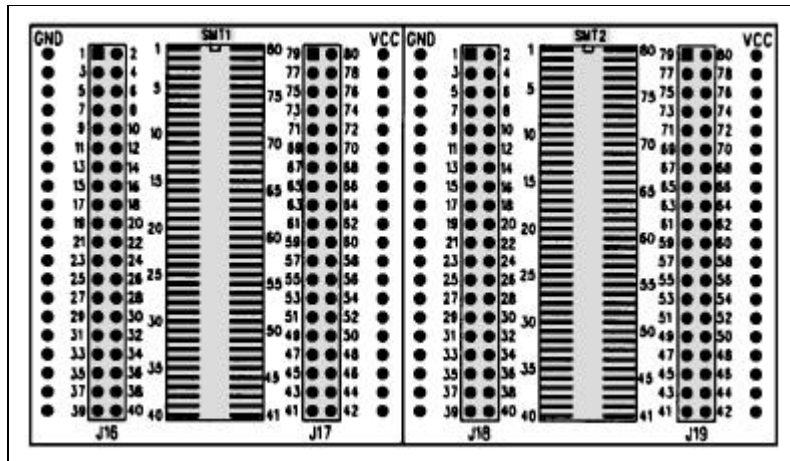
Figure 16: SMT Area
