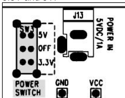
Figure 4: Power Switch
