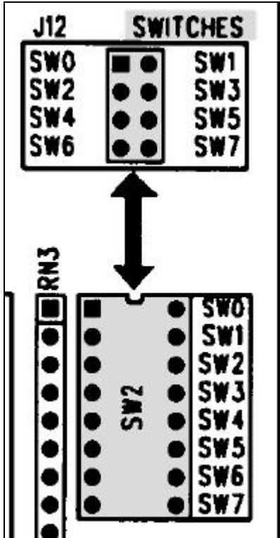
Figure 8: Switches
