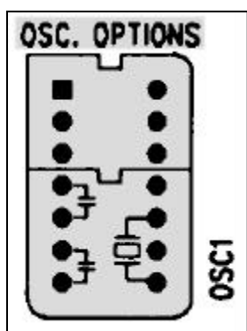
Figure 10: Oscillator Options
