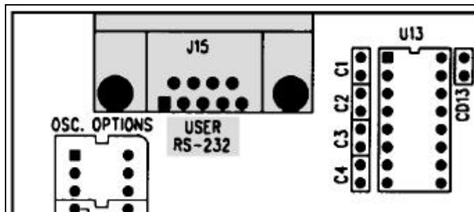
Figure 6: User RS-232 Connector
