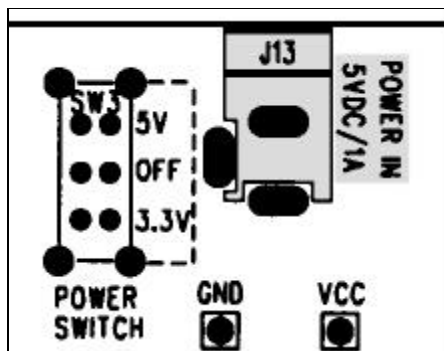
Figure 3: Power Connector
