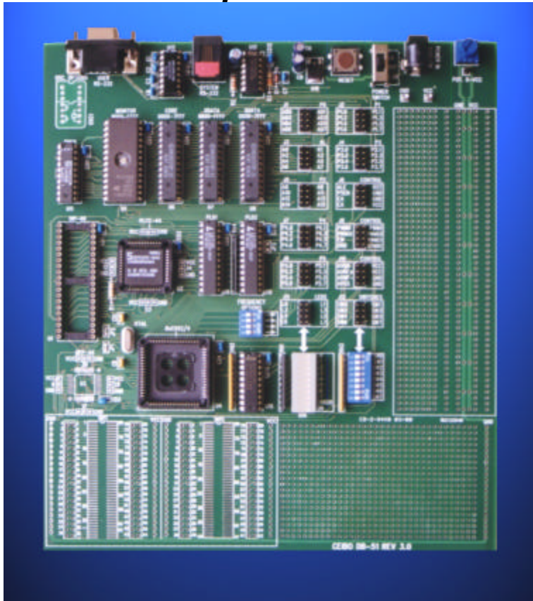
Development Board for Philips 80C51 Microcontrollers
