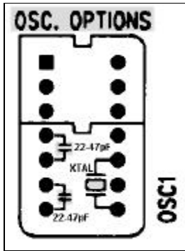
Figure 12: Crystal Option
