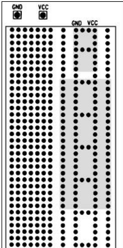
Figure 17: DIP Area
