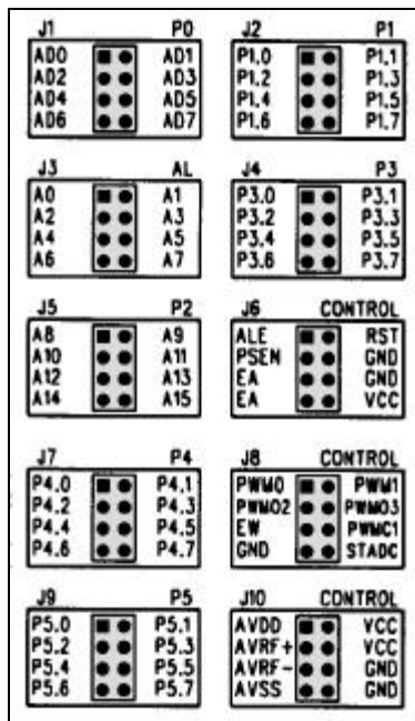
Figure 18: Microcontroller Signals
