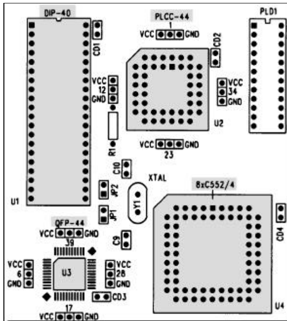
Figure 15: Microcontrollers
