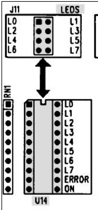
Figure 7: LEDs
