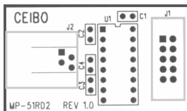
FIGURE 3: MP-51RD2 Programmer
