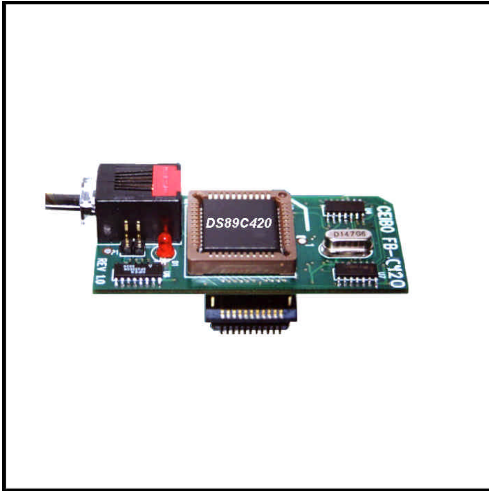
Development System for Dallas Semiconductors DS89C420 Microcontrollers
